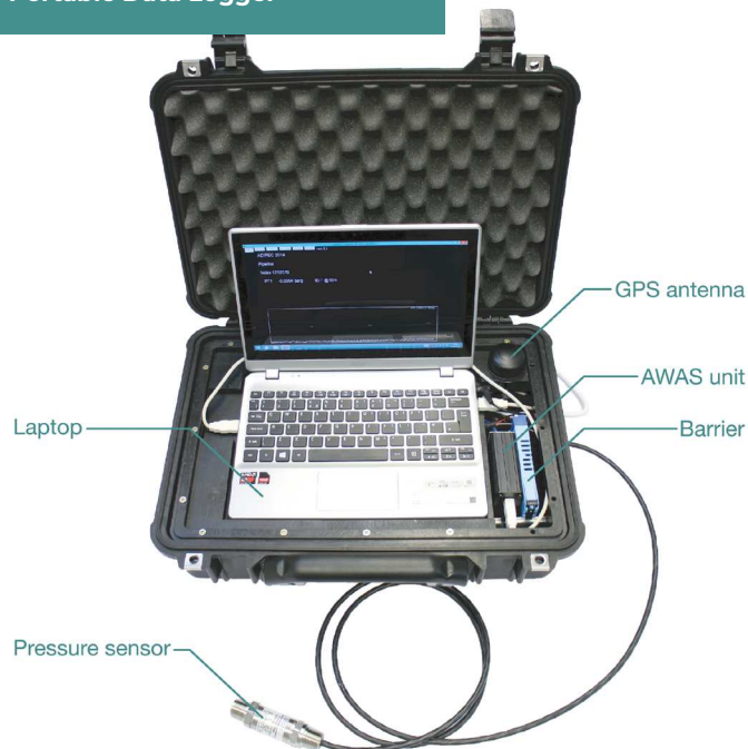
Portable Data Logger
